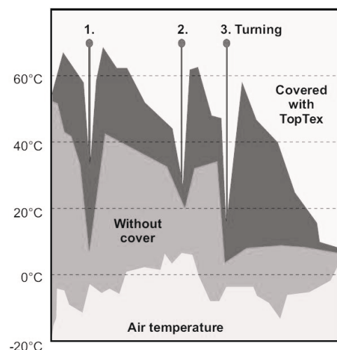
Temperature in test windrows
